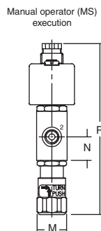
TYPE 03: Metal, epoxy coated / AISI 316L SS WP / WS: IEC 60335-1 EM / WSEM: EN/IEC 60079-7+18+31
