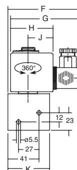
TYPE 04: Metal, epoxy coated / AISI 316L SS WP / WS: IEC 60335-1 EM / WSEM: EN/IEC 60079-7+18+31
