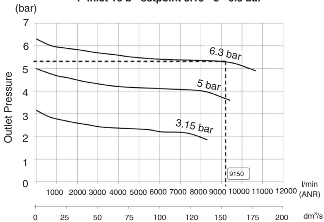
High Flow St. steel regulator 3/4" NPT Ref. : 342AA20D P inlet 10 b - setpoint 3.15 - 5 - 6.3 bar
