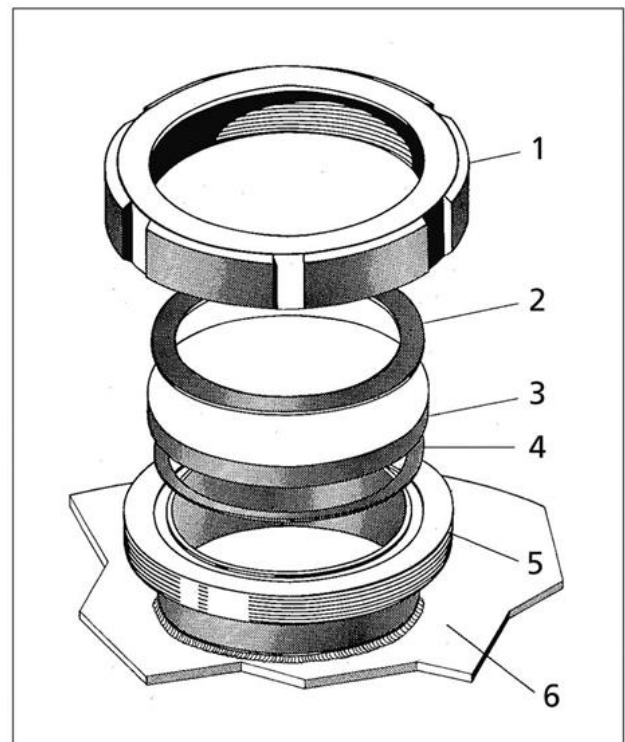
Components of screw-on sight glass
